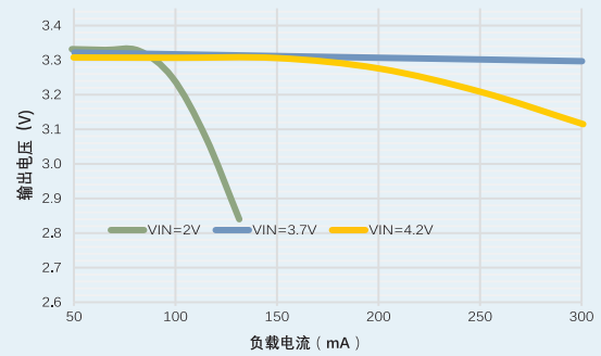
输出电压 vs. 负载电流
