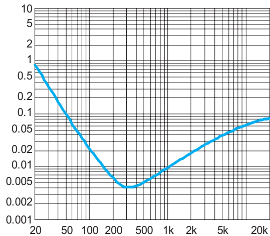
Figure 11. THD+N vs. Frequency SE mode, 6V, 320hm, P_o=70mW
