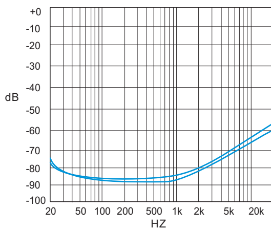
Figure 19. PSRR vs. Freq SE mode, 6V, 320hm, 200mVpp Input terminated
