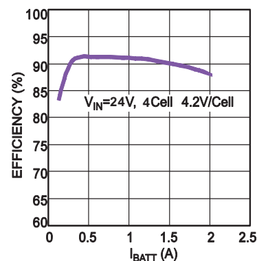
Efficiency Curve
