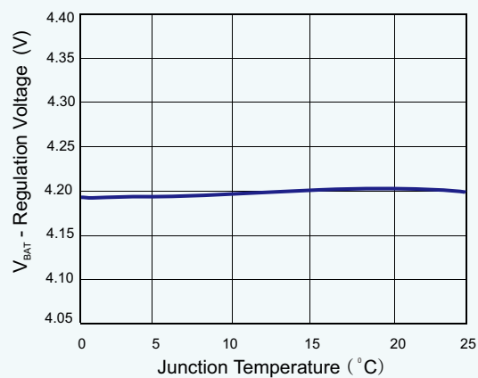
BAT Regulation Voltage vs Temperature
