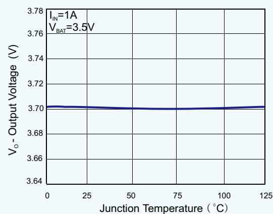
Output Regulation Voltage vs Temperature
