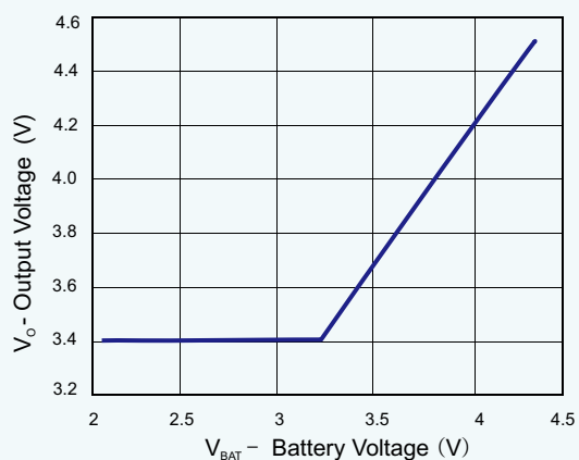
Output Regulation Voltage vs Battery Voltage
