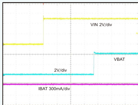
No Battery, No Load Power Up Timing
