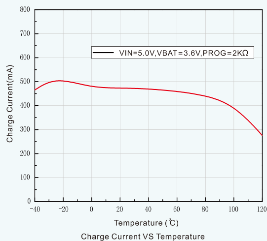
Charge Current VS Temperature
