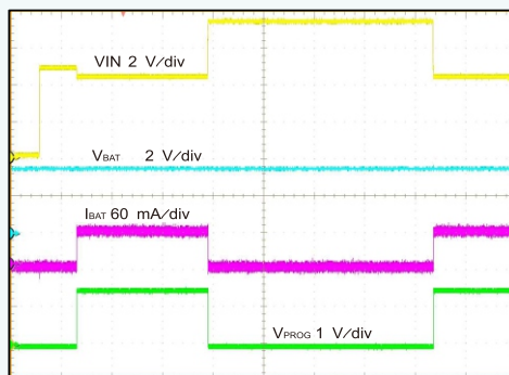
V IN 0V-5V-7V-5V OVP from Normal Power-Up Operation
