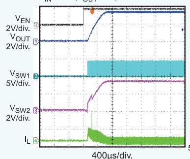
Power Up
