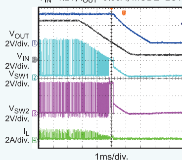
Power Off
