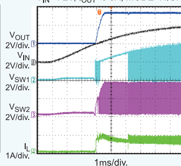
Power Up
