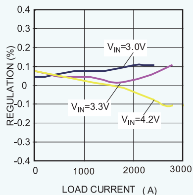
Load Regulation
