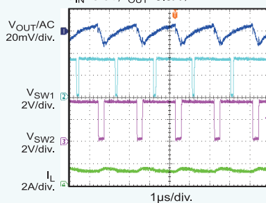
Steady State
