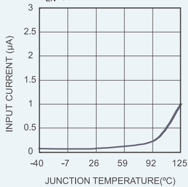
Disabled Supply Current vs. Temperature
