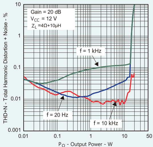
TOTAL HARMONIC DISTORTION + NOISE vs OUTPUT POWER
