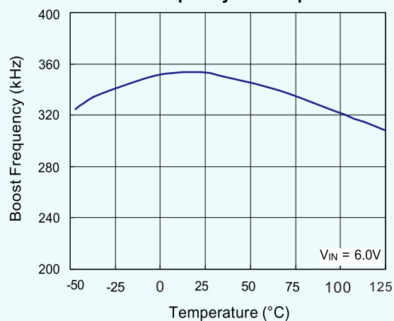
Boost Frequency vs. Temperature
