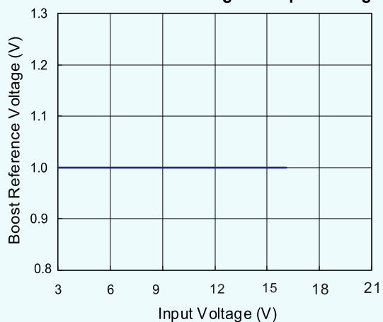
Boost Reference Voltage vs. Input Voltage
