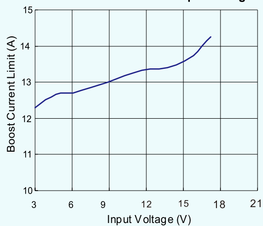
Boost Current Limit vs. Input Voltage
