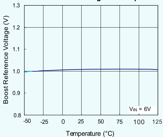
Boost Reference Voltage vs. Temperature
