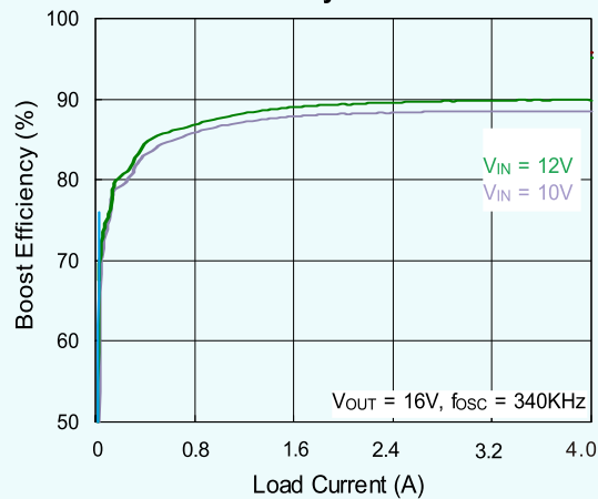
Boost Efficiency vs. Load Current
