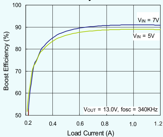
Boost Efficiency vs. Load Current
