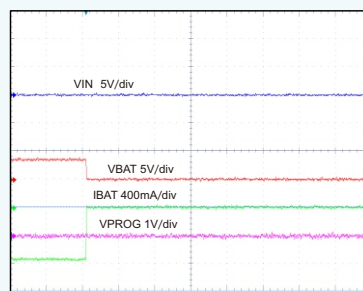
6- \Omega resistor at OUT, No input, V_{BAT} = 3.7\text{ V} Battery Removal
